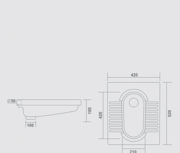
CITY PAN L 420 W 520 H 180mm
